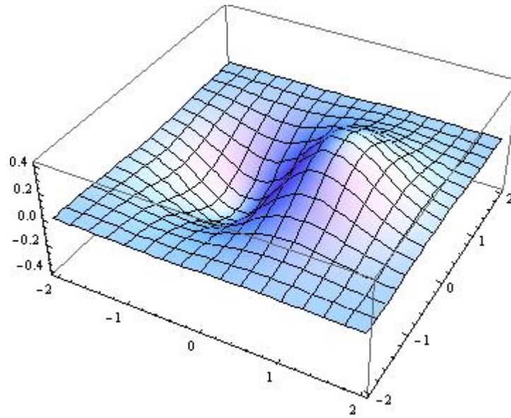
Plot3D
