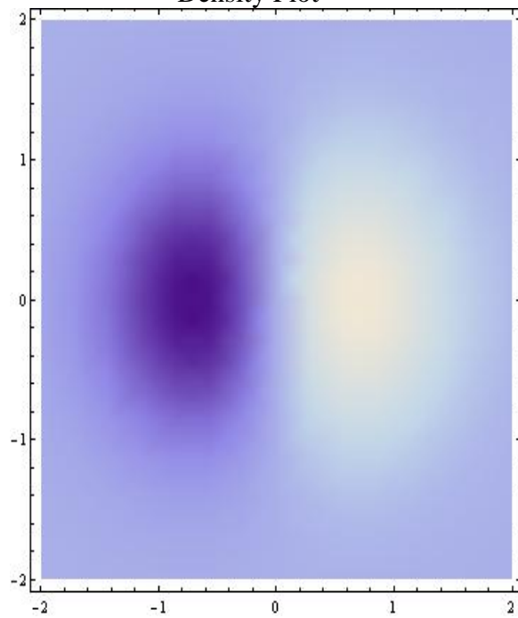
Density Plot
