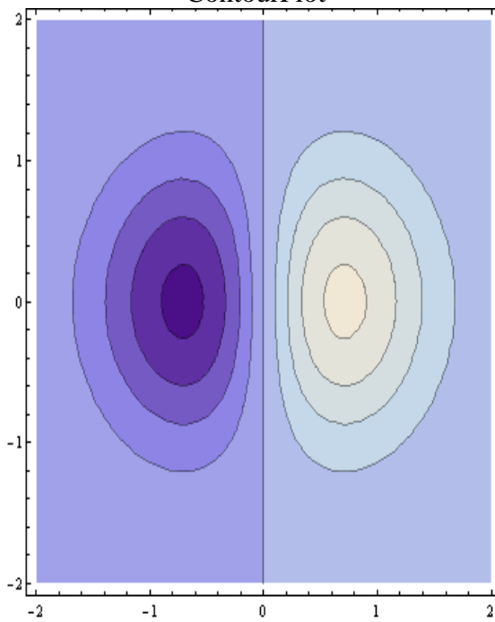
ContourPlot
