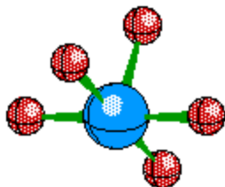
Square Pyramid
