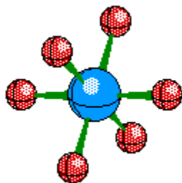
Octahedral
