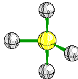
SeeSaw
