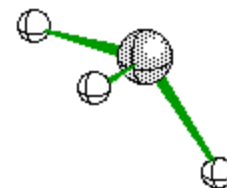
Trigonal Pyramid
