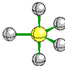
Trigonal Bipyramid
