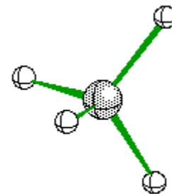
Tetrahedral
