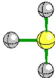
T-Shaped
